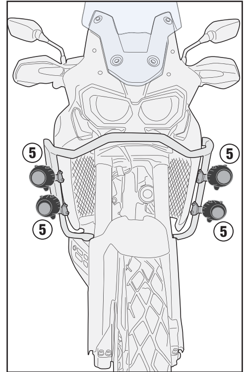
MOUNTING WITH 2 LS11610X
