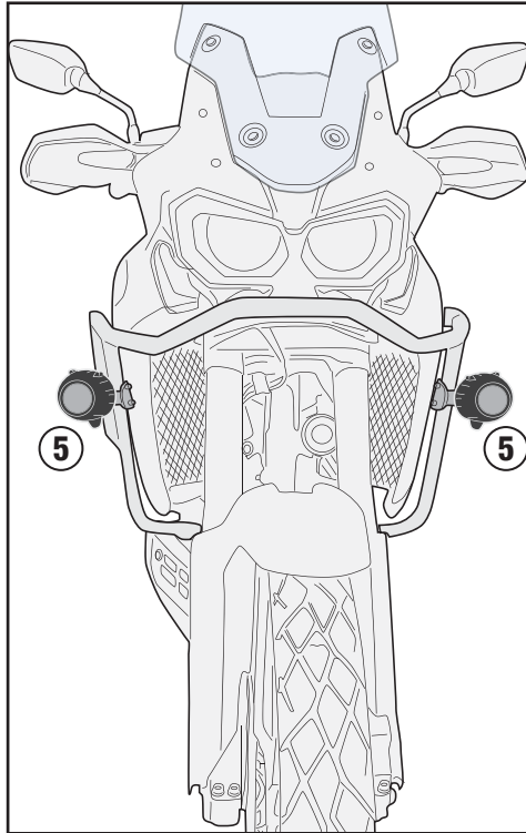
MOUNTING IN UPPER POSITION
